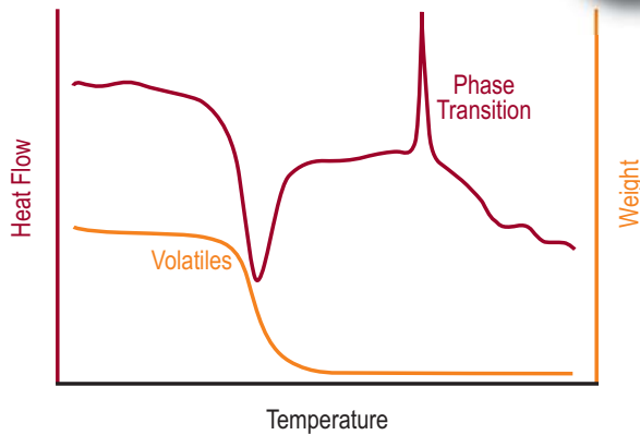
Simultaneous DSC/TGA
